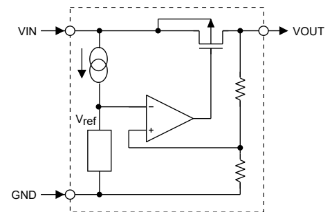
Block Diagram
